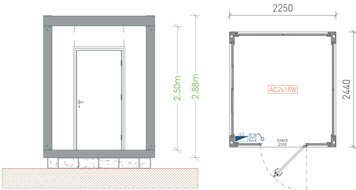
Main Elevation
