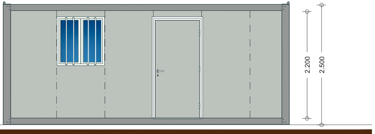
Main Elevation SCALE 1:50
