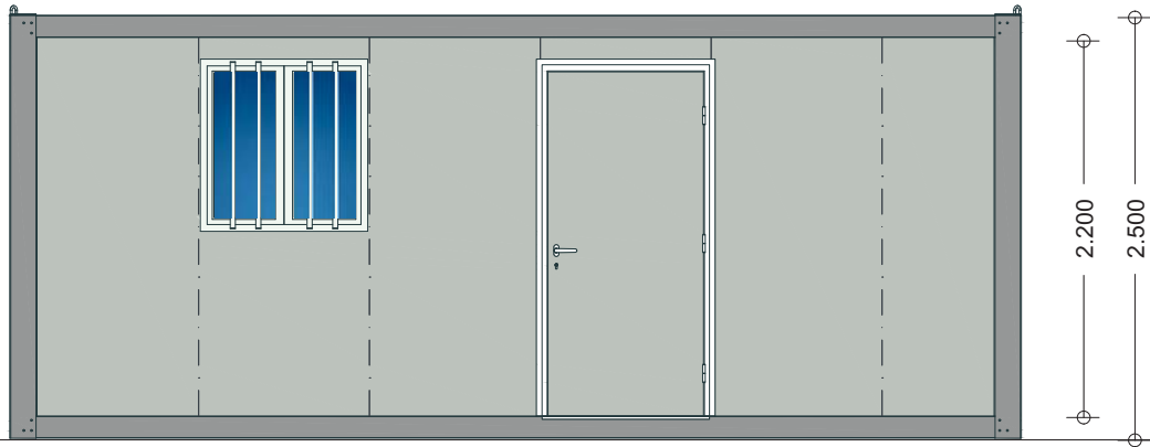
Main Elevation SCALE 1:50
