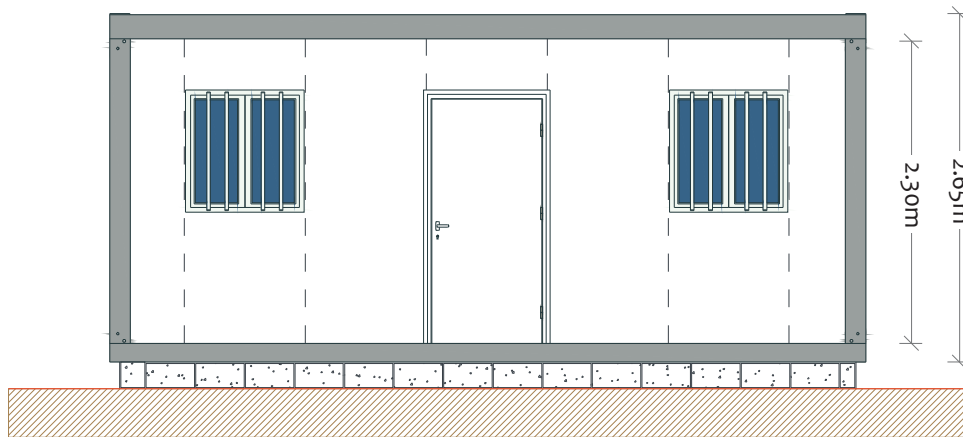
Main Elevation
