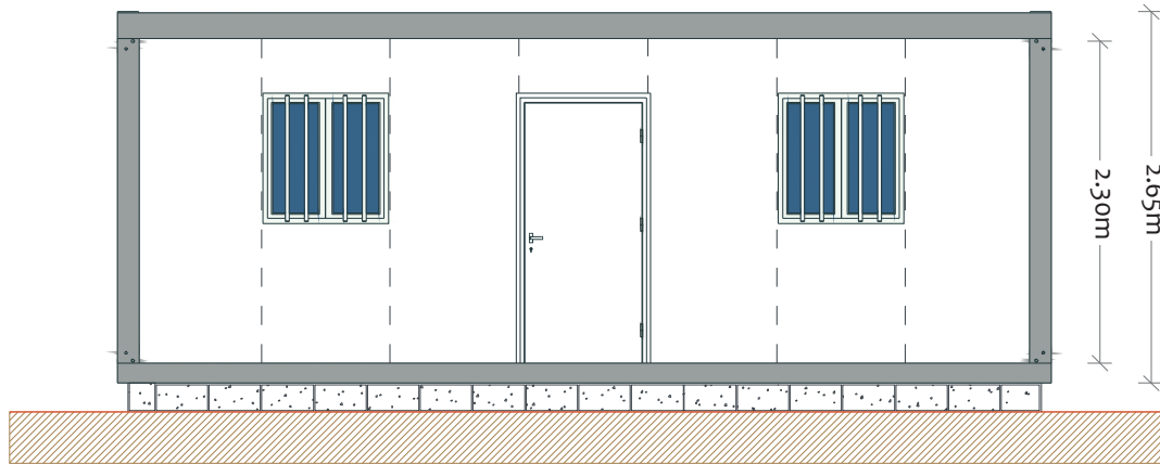
Main Elevation
